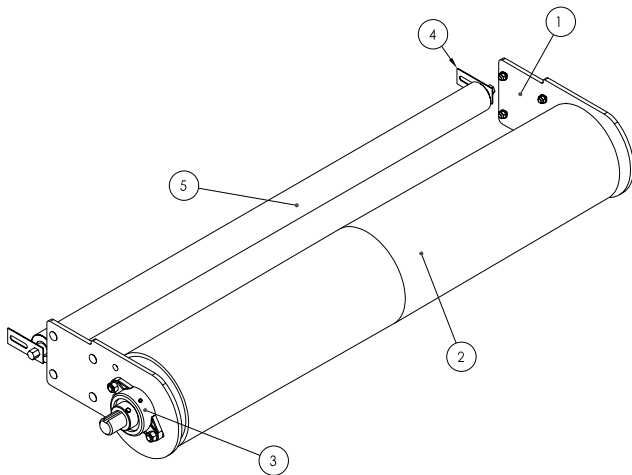
Figure 8.2 Drive Pulley
